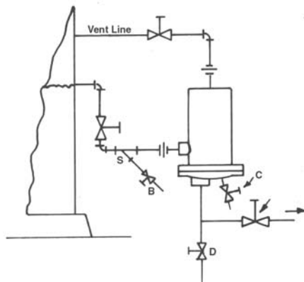
Figure 1. Installation of ball float drainer for medium or heavy loads. Strainer blow-down valve "B" and drainer blow-down valve "C" are optional. Discharge line valve "D" not required if drainer discharges water to ground.
